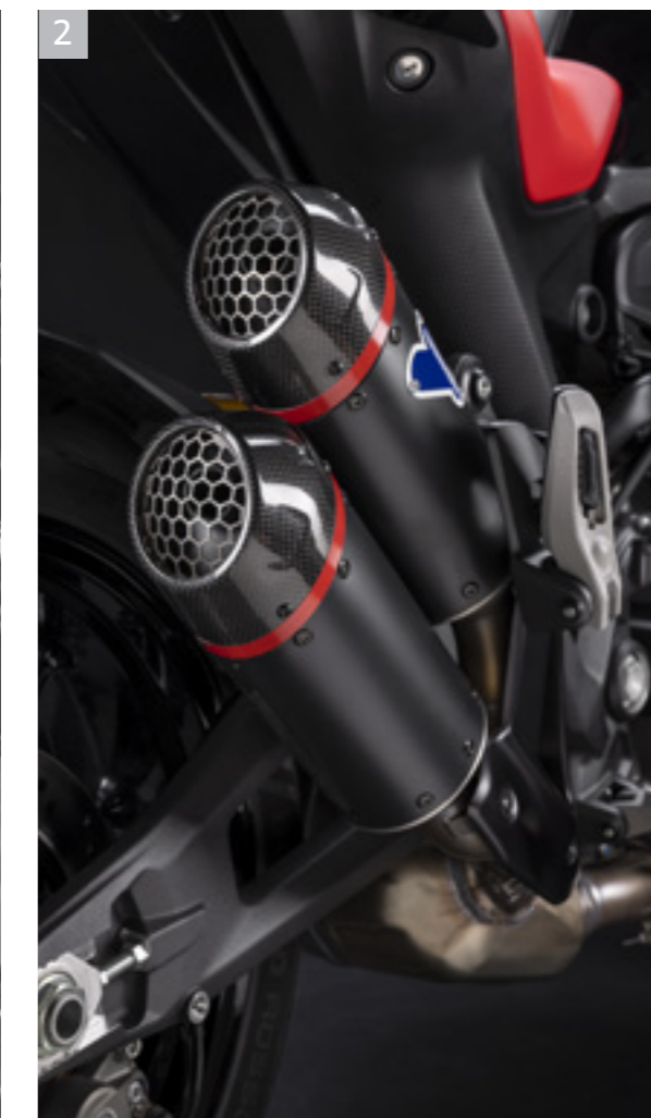
2 Pre-muffler and Termignoni type approved twin muffler, catalytic converter and 2 lambda probes
